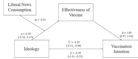
(b) Perceived effectiveness of vaccine as mediator, with conservative conversation as moderator
