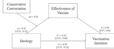
Figure 1. (a) Perceived effectiveness of vaccine as mediator, with liberal news consumption as moderator. (b) Perceived effectiveness of vaccine as mediator, with conservative conversation as moderator. Note (1): ideology is measured with a 5-point scale, with higher numbers indicating a more conservative ideology Note (2): effects presented in the figures do not involve demographics as control variables.
